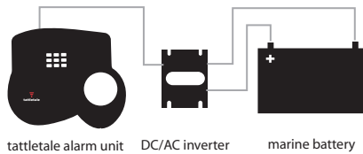
tattletale alarm unit DC/AC inverter marine battery
